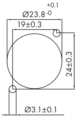
PANEL HOLE
